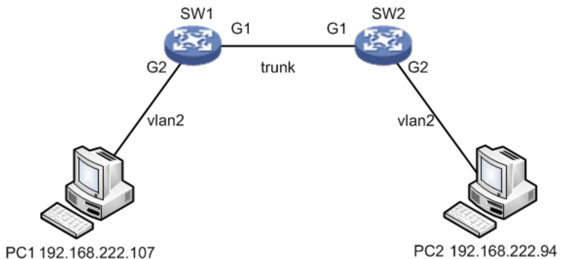
Figure 6-2 Networking
