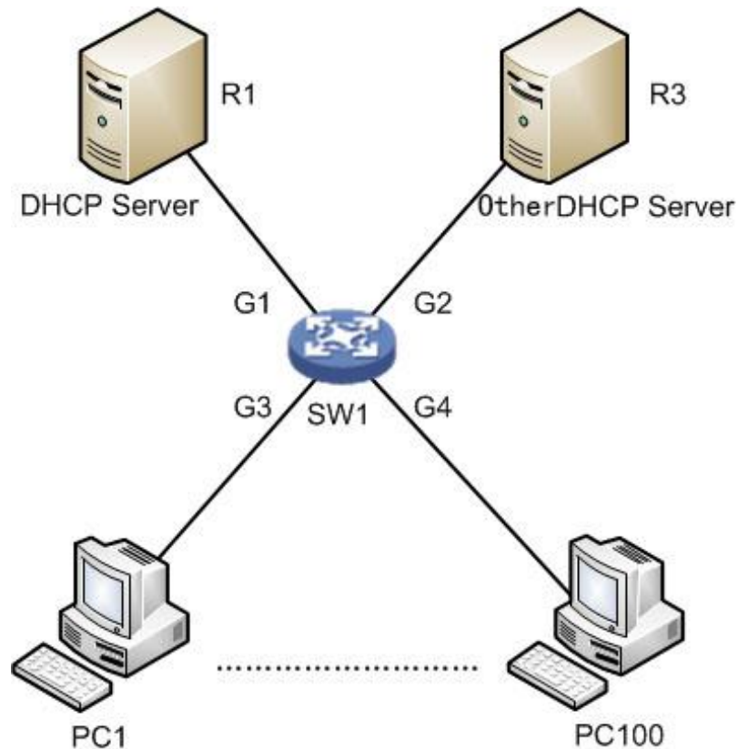
Figure 6-7 Networking
