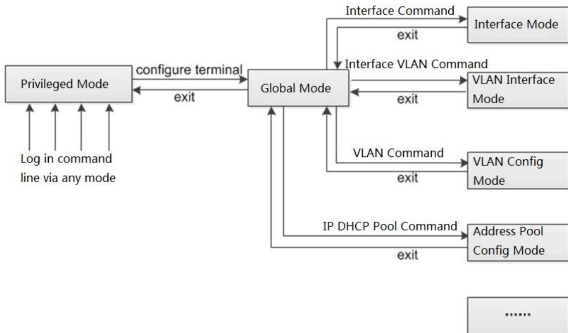
Figure 2-1 Layered structure for commamd mode
